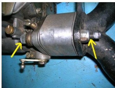
'Sealing 7' – Manifold / Carburettor
